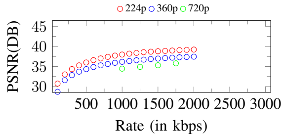
Figure 141. Curves of PSNR. Input: 720p, 2000Kbps
