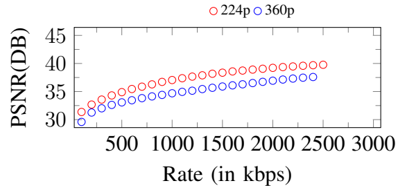
Figure 54. Curves of PSNR. Input: 360p, 2500Kbps
