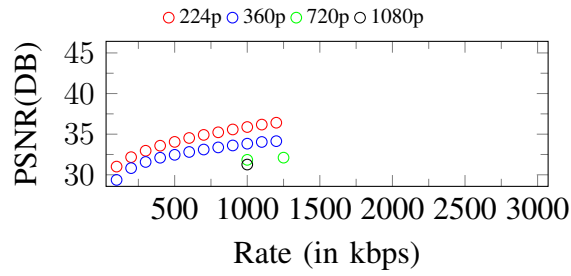
Figure 70. Curves of PSNR. Input: 1080p, 1250Kbps
