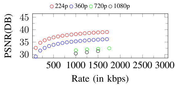
Figure 226. Curves of PSNR. Input: 1080p, 1750Kbps
