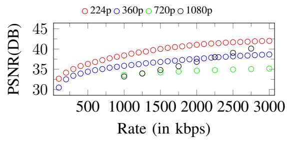
Figure 308. Curves of PSNR. Input: 1080p, 3000Kbps
