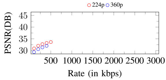
Figure 34. Curves of PSNR. Input: 360p, 500Kbps
