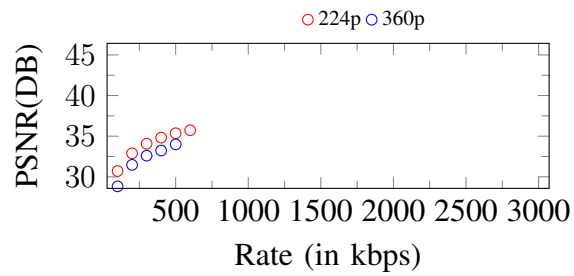
Figure 112. Curves of PSNR. Input: 360p, 600Kbps
