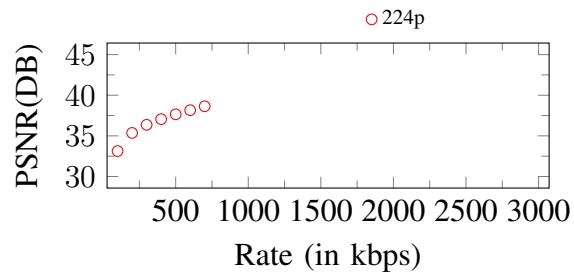
Figure 161. Curves of PSNR. Input: 224p, 800Kbps
