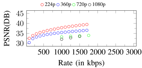
Figure 303. Curves of PSNR. Input: 1080p, 1750Kbps
