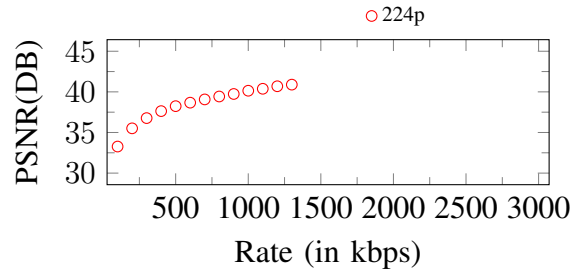
Figure 167. Curves of PSNR. Input: 224p, 1400Kbps
