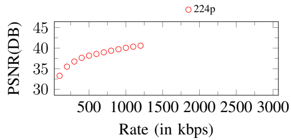
Figure 166. Curves of PSNR. Input: 224p, 1300Kbps
