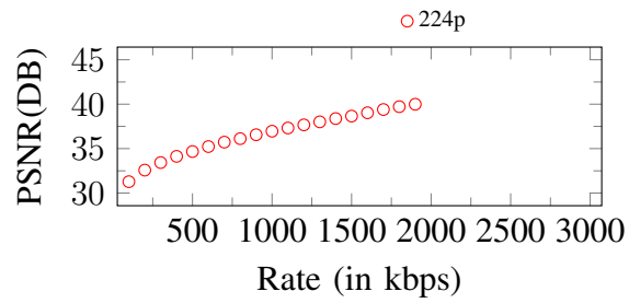
Figure 19. Curves of PSNR. Input: 224p, 2000Kbps
