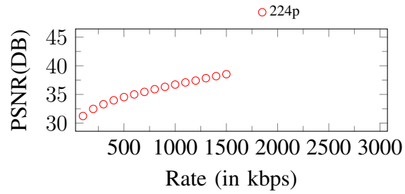
Figure 15. Curves of PSNR. Input: 224p, 1600Kbps
