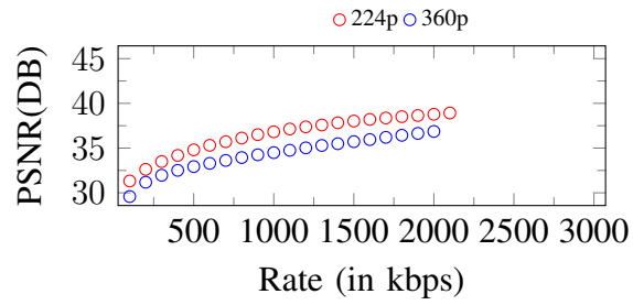
Figure 50. Curves of PSNR. Input: 360p, 2100Kbps
