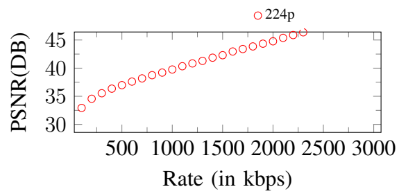
Figure 260. Curves of PSNR. Input: 224p, 3000Kbps
