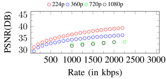
Figure 74. Curves of PSNR. Input: 1080p, 2250Kbps
