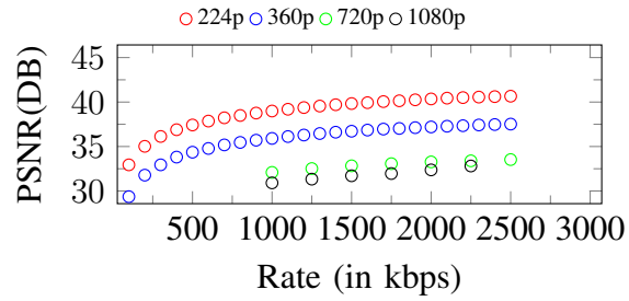
Figure 229. Curves of PSNR. Input: 1080p, 2500Kbps
