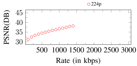
Figure 14. Curves of PSNR. Input: 224p, 1500Kbps
