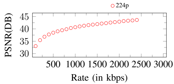
Figure 178. Curves of PSNR. Input: 224p, 2500Kbps
