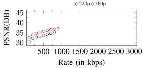
Figure 269. Curves of PSNR. Input: 360p, 900Kbps
