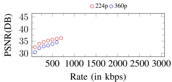
Figure 267. Curves of PSNR. Input: 360p, 700Kbps
