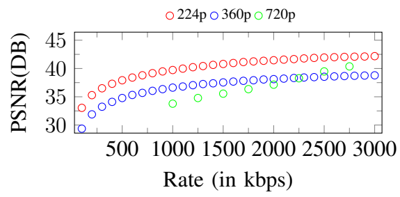
Figure 222. Curves of PSNR. Input: 720p, 3000Kbps
