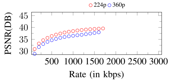
Figure 123. Curves of PSNR. Input: 360p, 1700Kbps
