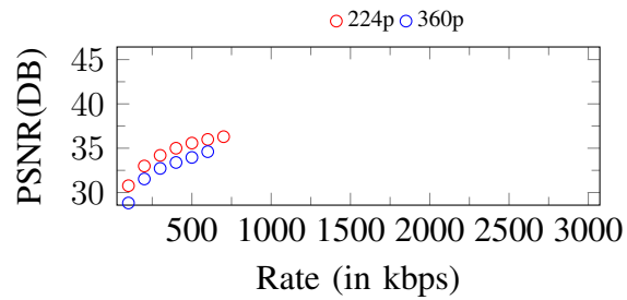
Figure 113. Curves of PSNR. Input: 360p, 700Kbps
