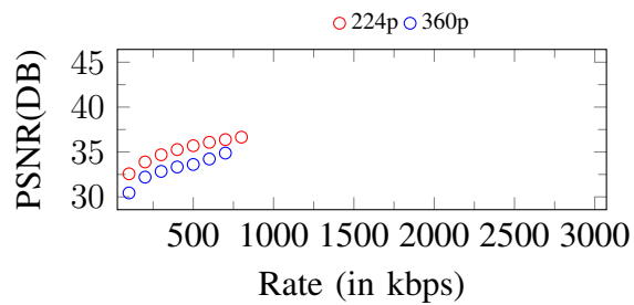
Figure 268. Curves of PSNR. Input: 360p, 800Kbps
