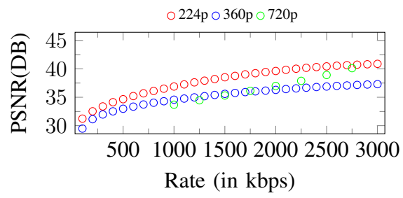
Figure 68. Curves of PSNR. Input: 720p, 3000Kbps
