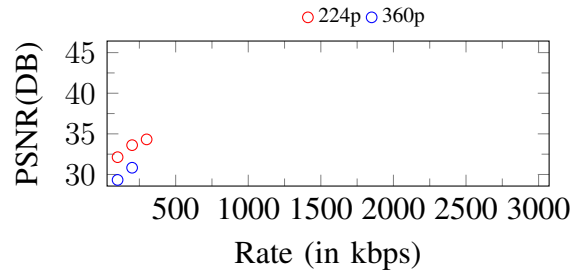
Figure 186. Curves of PSNR. Input: 360p, 300Kbps
