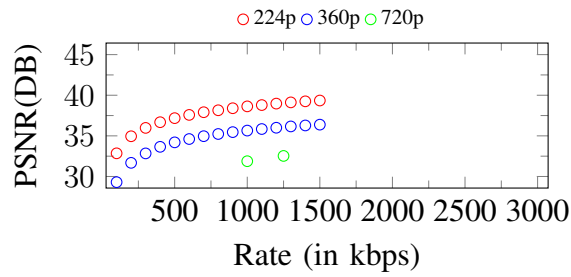
Figure 216. Curves of PSNR. Input: 720p, 1500Kbps
