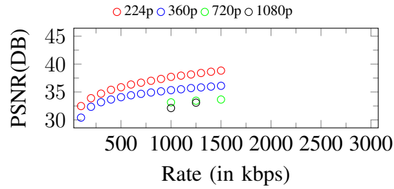
Figure 302. Curves of PSNR. Input: 1080p, 1500Kbps
