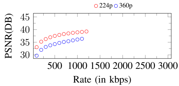
Figure 195. Curves of PSNR. Input: 360p, 1200Kbps
