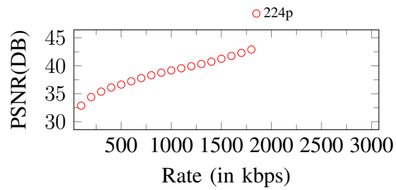
Figure 249. Curves of PSNR. Input: 224p, 1900Kbps
