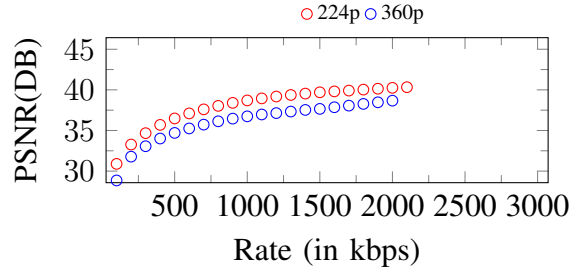
Figure 127. Curves of PSNR. Input: 360p, 2100Kbps
