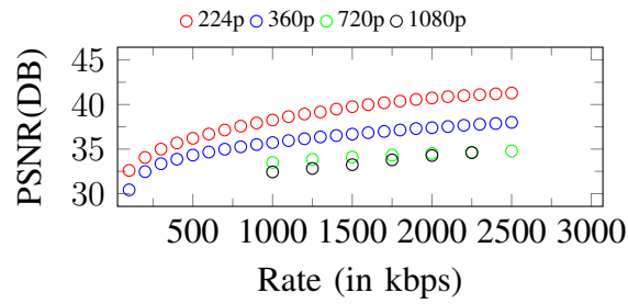
Figure 306. Curves of PSNR. Input: 1080p, 2500Kbps
