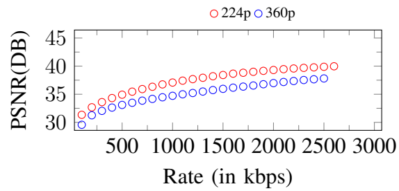
Figure 55. Curves of PSNR. Input: 360p, 2600Kbps
