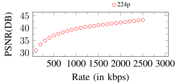
Figure 102. Curves of PSNR. Input: 224p, 2600Kbps
