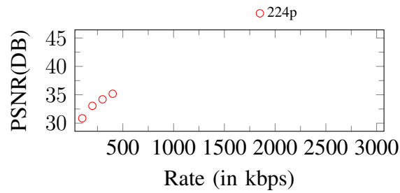
Figure 81. Curves of PSNR. Input: 224p, 500Kbps
