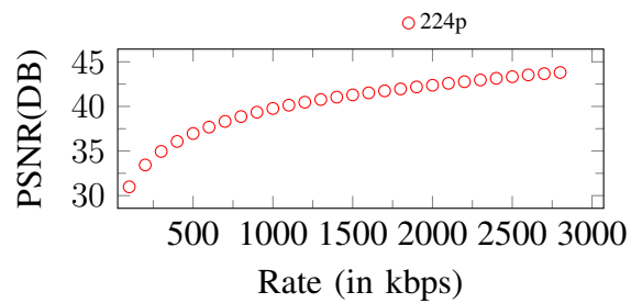
Figure 105. Curves of PSNR. Input: 224p, 2900Kbps
