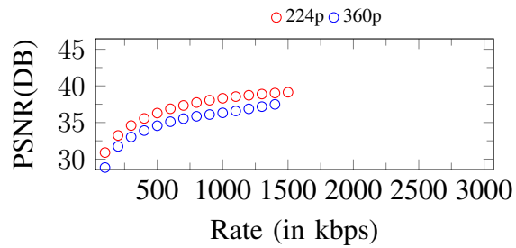
Figure 121. Curves of PSNR. Input: 360p, 1500Kbps
