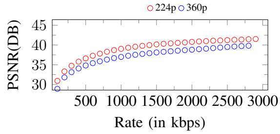
Figure 135. Curves of PSNR. Input: 360p, 2900Kbps
