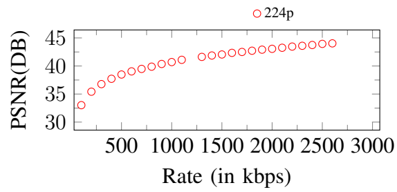
Figure 180. Curves of PSNR. Input: 224p, 2700Kbps
