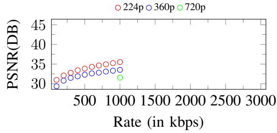
Figure 69. Curves of PSNR. Input: 1080p, 1000Kbps
