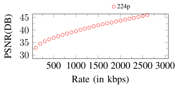
Figure 257. Curves of PSNR. Input: 224p, 2700Kbps
