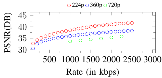
Figure 297. Curves of PSNR. Input: 720p, 2500Kbps
