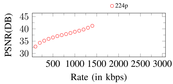
Figure 245. Curves of PSNR. Input: 224p, 1500Kbps
