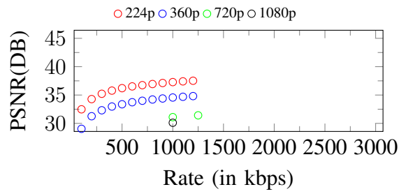
Figure 224. Curves of PSNR. Input: 1080p, 1250Kbps
