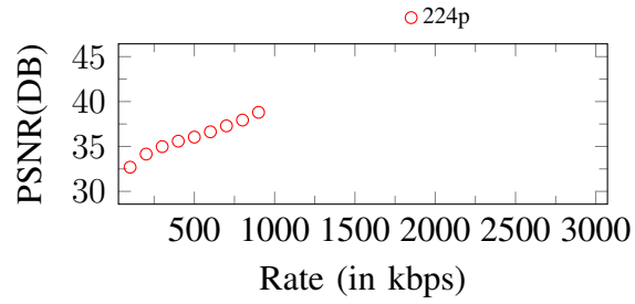
Figure 240. Curves of PSNR. Input: 224p, 1000Kbps
