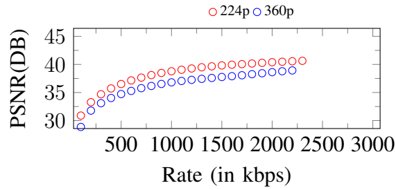
Figure 129. Curves of PSNR. Input: 360p, 2300Kbps
