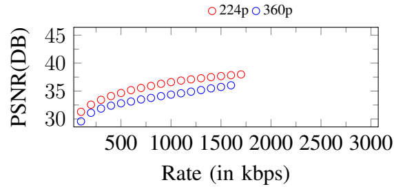
Figure 46. Curves of PSNR. Input: 360p, 1700Kbps
