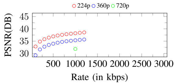
Figure 215. Curves of PSNR. Input: 720p, 1250Kbps
