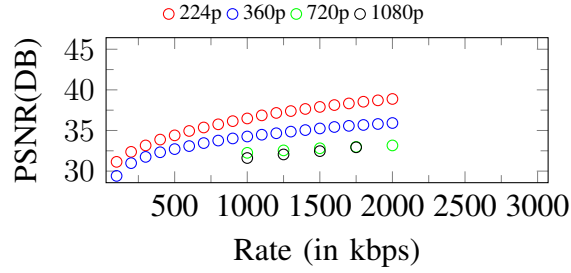
Figure 73. Curves of PSNR. Input: 1080p, 2000Kbps
