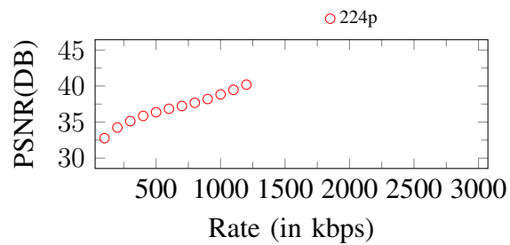
Figure 243. Curves of PSNR. Input: 224p, 1300Kbps
