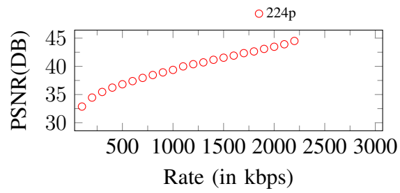
Figure 253. Curves of PSNR. Input: 224p, 2300Kbps
