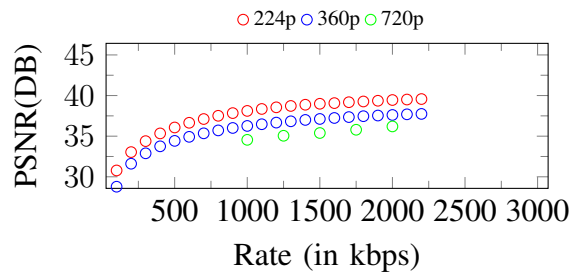
Figure 142. Curves of PSNR. Input: 720p, 2250Kbps
