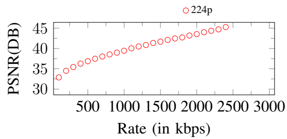
Figure 255. Curves of PSNR. Input: 224p, 2500Kbps
