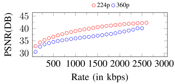
Figure 286. Curves of PSNR. Input: 360p, 2600Kbps
