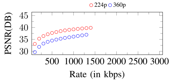
Figure 197. Curves of PSNR. Input: 360p, 1400Kbps
