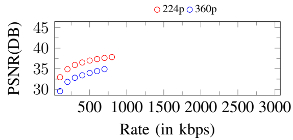
Figure 191. Curves of PSNR. Input: 360p, 800Kbps
