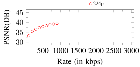
Figure 163. Curves of PSNR. Input: 224p, 1000Kbps
