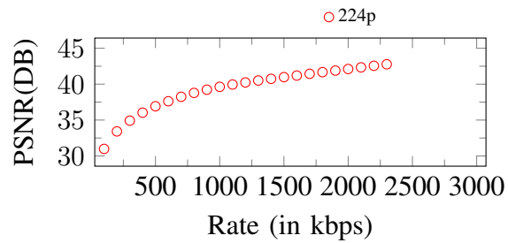
Figure 100. Curves of PSNR. Input: 224p, 2400Kbps
