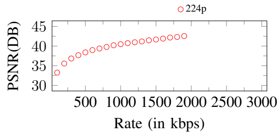
Figure 173. Curves of PSNR. Input: 224p, 2000Kbps
