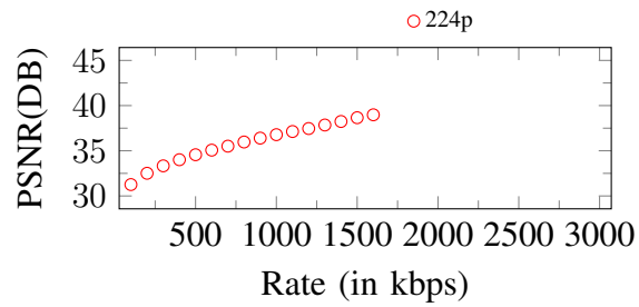
Figure 16. Curves of PSNR. Input: 224p, 1700Kbps
