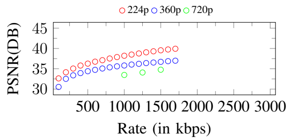
Figure 294. Curves of PSNR. Input: 720p, 1750Kbps
