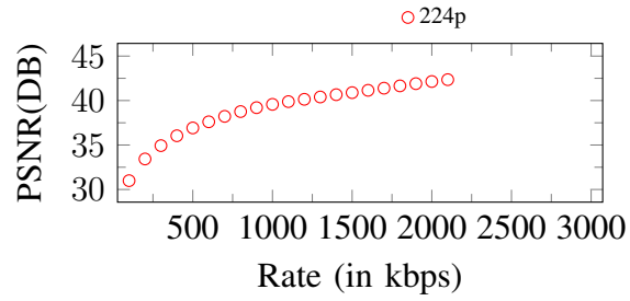
Figure 98. Curves of PSNR. Input: 224p, 2200Kbps
