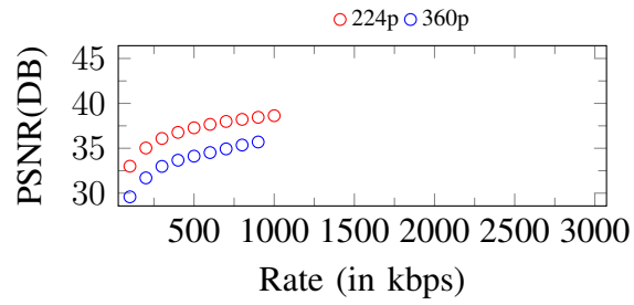
Figure 193. Curves of PSNR. Input: 360p, 1000Kbps
