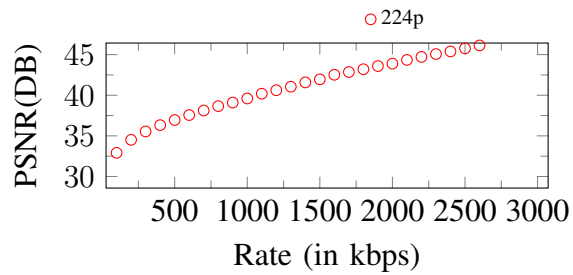
Figure 258. Curves of PSNR. Input: 224p, 2800Kbps
