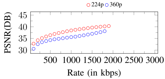
Figure 279. Curves of PSNR. Input: 360p, 1900Kbps
