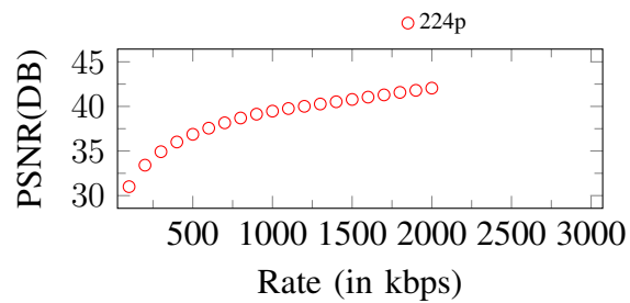
Figure 97. Curves of PSNR. Input: 224p, 2100Kbps
