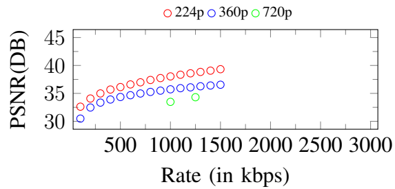
Figure 293. Curves of PSNR. Input: 720p, 1500Kbps
