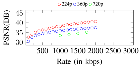
Figure 295. Curves of PSNR. Input: 720p, 2000Kbps
