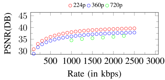
Figure 143. Curves of PSNR. Input: 720p, 2500Kbps
