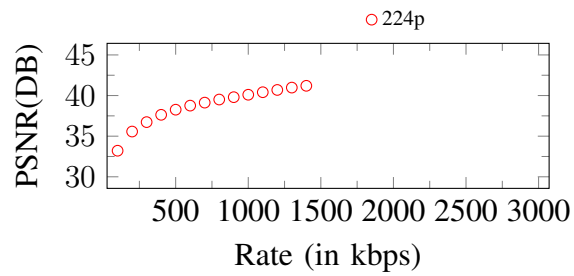
Figure 168. Curves of PSNR. Input: 224p, 1500Kbps
