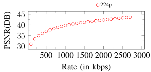
Figure 104. Curves of PSNR. Input: 224p, 2800Kbps
