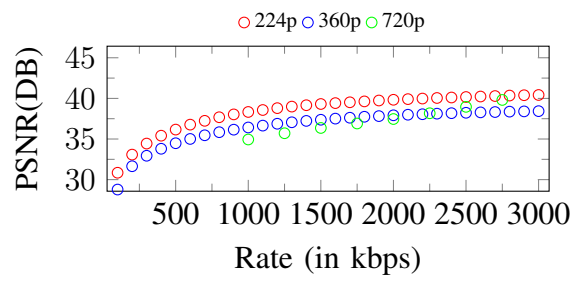
Figure 145. Curves of PSNR. Input: 720p, 3000Kbps
