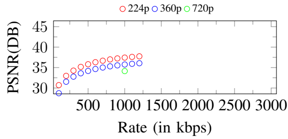
Figure 138. Curves of PSNR. Input: 720p, 1250Kbps
