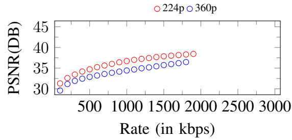
Figure 48. Curves of PSNR. Input: 360p, 1900Kbps
