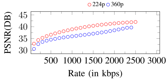
Figure 285. Curves of PSNR. Input: 360p, 2500Kbps
