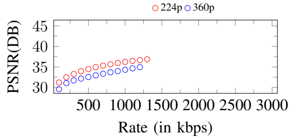
Figure 42. Curves of PSNR. Input: 360p, 1300Kbps
