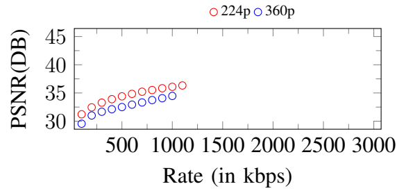
Figure 40. Curves of PSNR. Input: 360p, 1100Kbps
