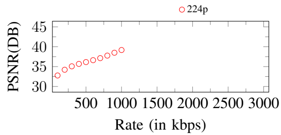
Figure 241. Curves of PSNR. Input: 224p, 1100Kbps
