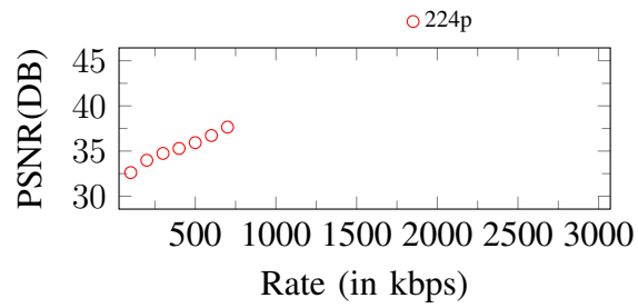
Figure 238. Curves of PSNR. Input: 224p, 800Kbps
