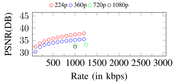
Figure 301. Curves of PSNR. Input: 1080p, 1250Kbps
