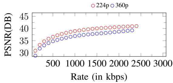
Figure 130. Curves of PSNR. Input: 360p, 2400Kbps
