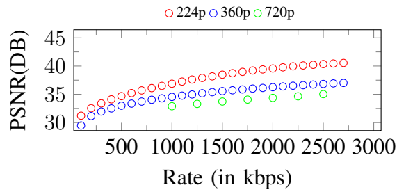
Figure 67. Curves of PSNR. Input: 720p, 2750Kbps
