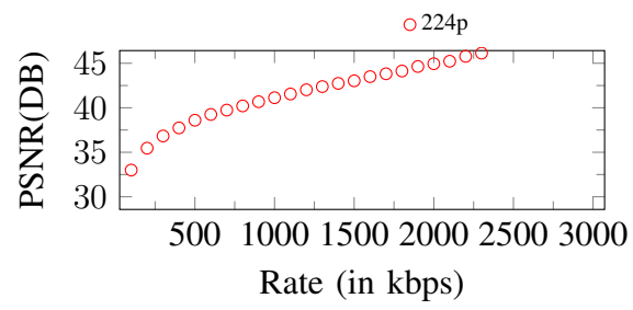
Figure 183. Curves of PSNR. Input: 224p, 3000Kbps
