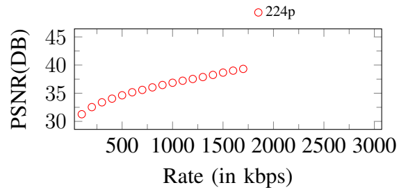
Figure 17. Curves of PSNR. Input: 224p, 1800Kbps
