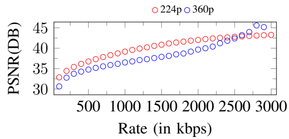
Figure 290. Curves of PSNR. Input: 360p, 3000Kbps
