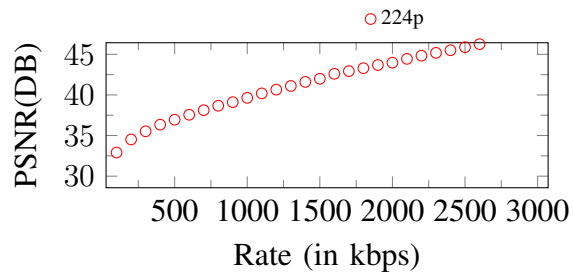
Figure 259. Curves of PSNR. Input: 224p, 2900Kbps
