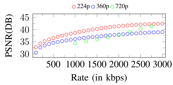
Figure 299. Curves of PSNR. Input: 720p, 3000Kbps
