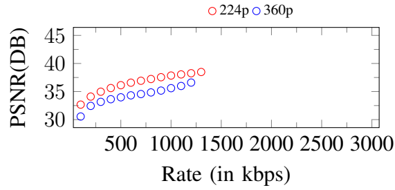
Figure 273. Curves of PSNR. Input: 360p, 1300Kbps
