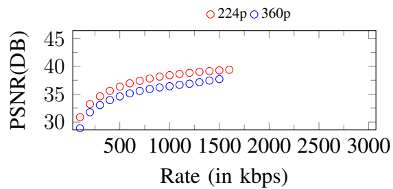
Figure 122. Curves of PSNR. Input: 360p, 1600Kbps
