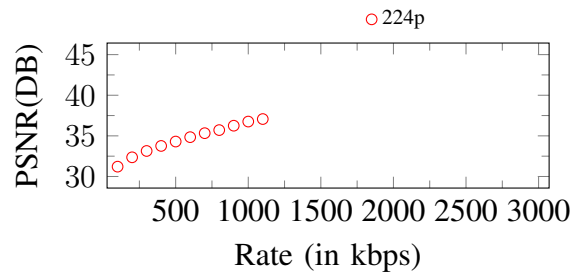
Figure 11. Curves of PSNR. Input: 224p, 1200Kbps
