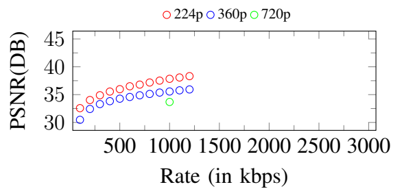
Figure 292. Curves of PSNR. Input: 720p, 1250Kbps
