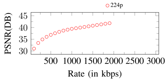
Figure 96. Curves of PSNR. Input: 224p, 2000Kbps
