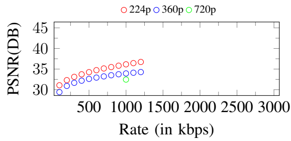
Figure 61. Curves of PSNR. Input: 720p, 1250Kbps
