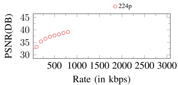
Figure 162. Curves of PSNR. Input: 224p, 900Kbps
