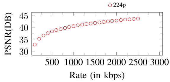
Figure 179. Curves of PSNR. Input: 224p, 2600Kbps
