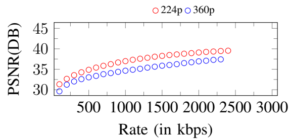
Figure 53. Curves of PSNR. Input: 360p, 2400Kbps
