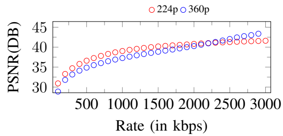
Figure 136. Curves of PSNR. Input: 360p, 3000Kbps
