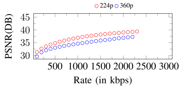
Figure 52. Curves of PSNR. Input: 360p, 2300Kbps
