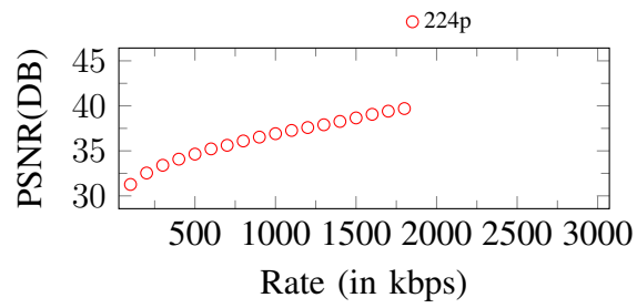
Figure 18. Curves of PSNR. Input: 224p, 1900Kbps
