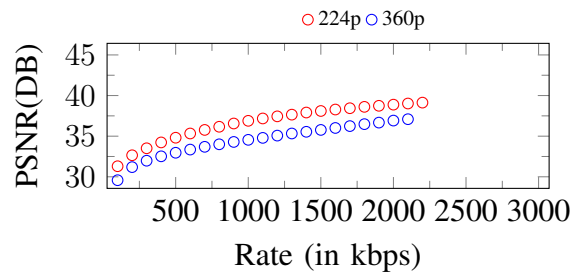
Figure 51. Curves of PSNR. Input: 360p, 2200Kbps
