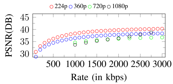
Figure 154. Curves of PSNR. Input: 1080p, 3000Kbps
