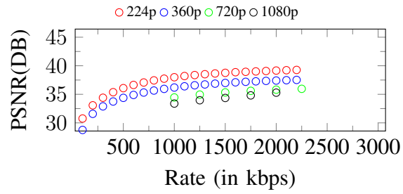
Figure 151. Curves of PSNR. Input: 1080p, 2250Kbps
