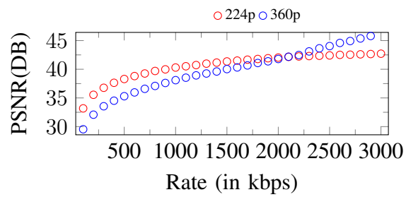
Figure 213. Curves of PSNR. Input: 360p, 3000Kbps
