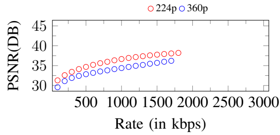
Figure 47. Curves of PSNR. Input: 360p, 1800Kbps
