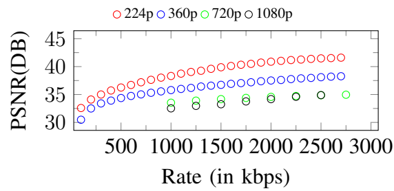
Figure 307. Curves of PSNR. Input: 1080p, 2750Kbps
