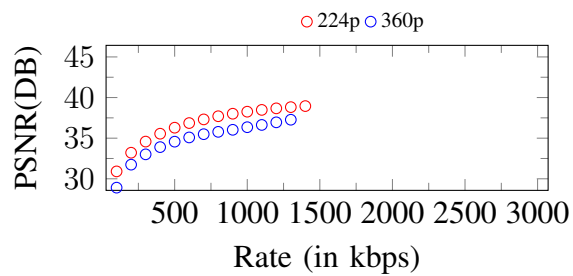
Figure 120. Curves of PSNR. Input: 360p, 1400Kbps
