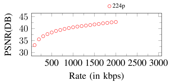
Figure 174. Curves of PSNR. Input: 224p, 2100Kbps
