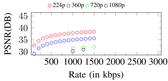
Figure 225. Curves of PSNR. Input: 1080p, 1500Kbps
