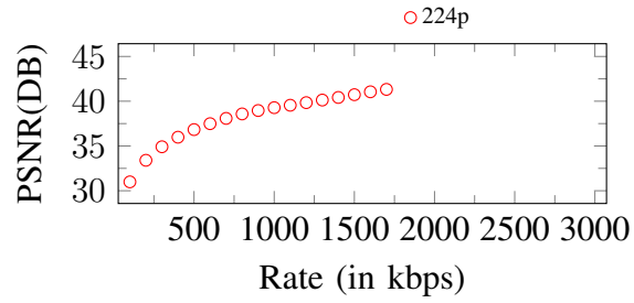
Figure 94. Curves of PSNR. Input: 224p, 1800Kbps
