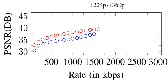
Figure 276. Curves of PSNR. Input: 360p, 1600Kbps
