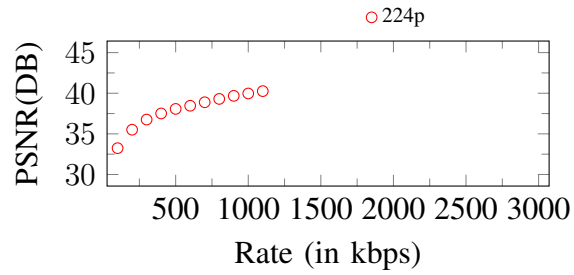
Figure 165. Curves of PSNR. Input: 224p, 1200Kbps
