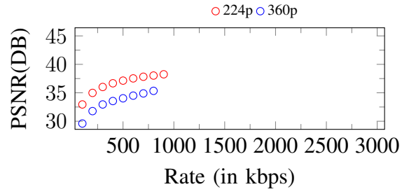
Figure 192. Curves of PSNR. Input: 360p, 900Kbps
