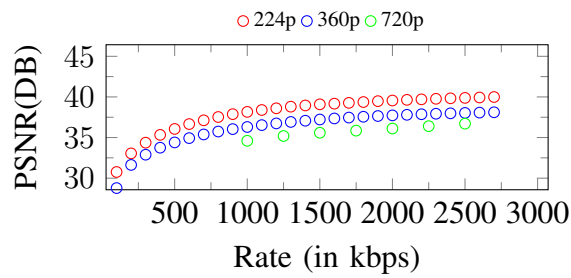
Figure 144. Curves of PSNR. Input: 720p, 2750Kbps
