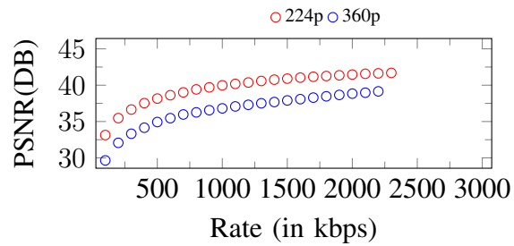
Figure 206. Curves of PSNR. Input: 360p, 2300Kbps
