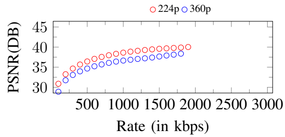
Figure 125. Curves of PSNR. Input: 360p, 1900Kbps
