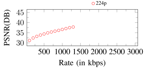
Figure 13. Curves of PSNR. Input: 224p, 1400Kbps
