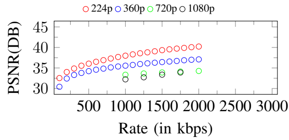
Figure 304. Curves of PSNR. Input: 1080p, 2000Kbps
