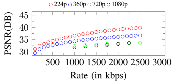
Figure 75. Curves of PSNR. Input: 1080p, 2500Kbps
