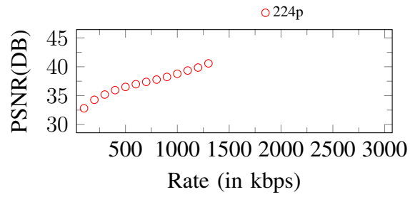
Figure 244. Curves of PSNR. Input: 224p, 1400Kbps
