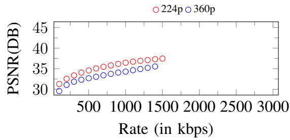
Figure 44. Curves of PSNR. Input: 360p, 1500Kbps
