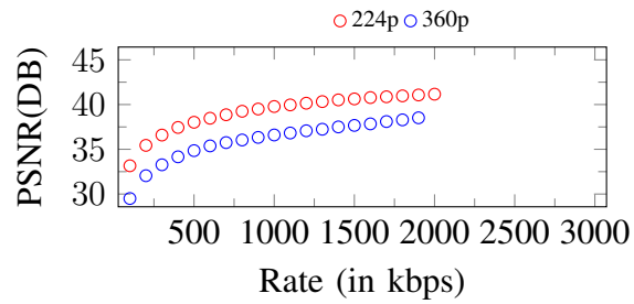
Figure 203. Curves of PSNR. Input: 360p, 2000Kbps
