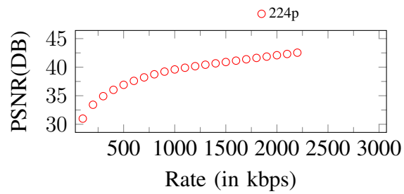
Figure 99. Curves of PSNR. Input: 224p, 2300Kbps
