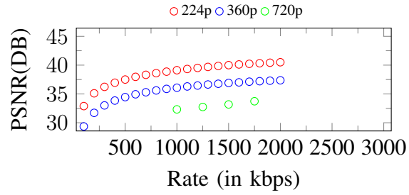
Figure 218. Curves of PSNR. Input: 720p, 2000Kbps
