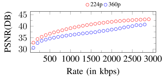
Figure 289. Curves of PSNR. Input: 360p, 2900Kbps
