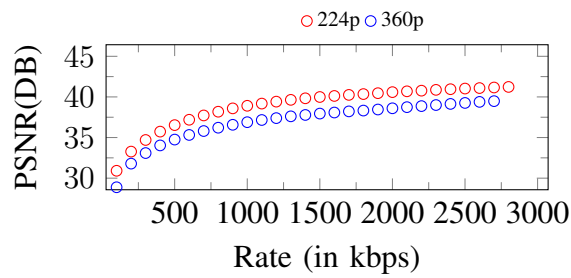
Figure 134. Curves of PSNR. Input: 360p, 2800Kbps
