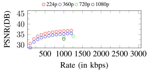
Figure 147. Curves of PSNR. Input: 1080p, 1250Kbps
