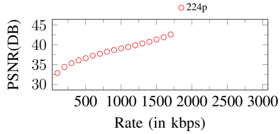
Figure 248. Curves of PSNR. Input: 224p, 1800Kbps
