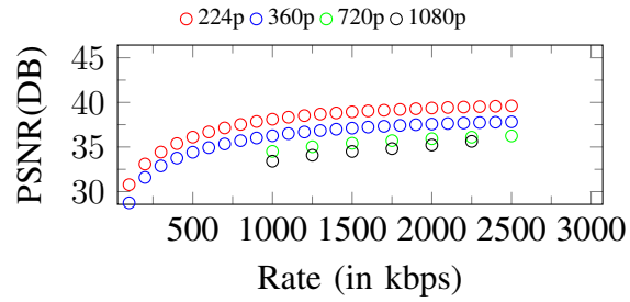
Figure 152. Curves of PSNR. Input: 1080p, 2500Kbps
