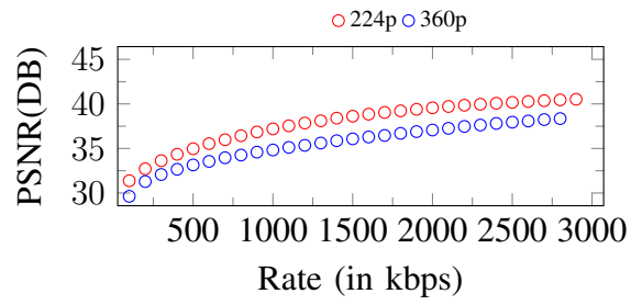
Figure 58. Curves of PSNR. Input: 360p, 2900Kbps
