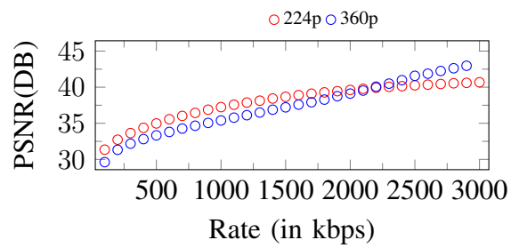
Figure 59. Curves of PSNR. Input: 360p, 3000Kbps
