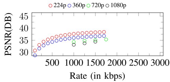
Figure 149. Curves of PSNR. Input: 1080p, 1750Kbps
