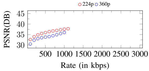
Figure 271. Curves of PSNR. Input: 360p, 1100Kbps
