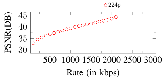
Figure 252. Curves of PSNR. Input: 224p, 2200Kbps
