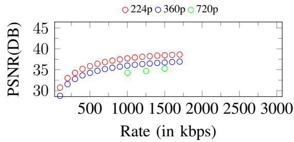
Figure 140. Curves of PSNR. Input: 720p, 1750Kbps
