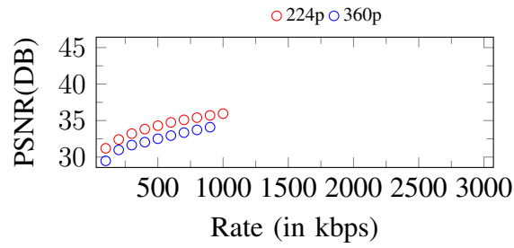
Figure 39. Curves of PSNR. Input: 360p, 1000Kbps
