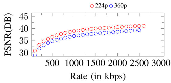
Figure 132. Curves of PSNR. Input: 360p, 2600Kbps
