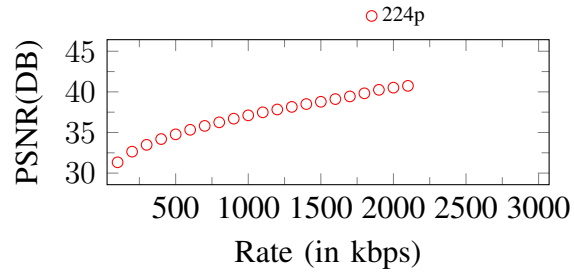
Figure 21. Curves of PSNR. Input: 224p, 2200Kbps
