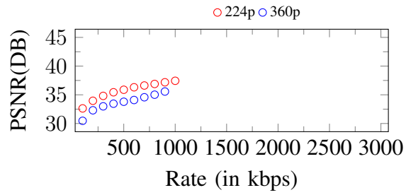
Figure 270. Curves of PSNR. Input: 360p, 1000Kbps
