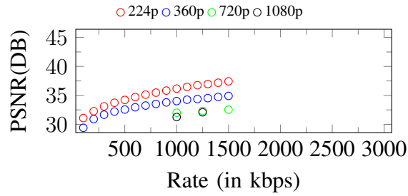
Figure 71. Curves of PSNR. Input: 1080p, 1500Kbps
