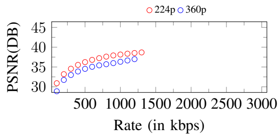
Figure 119. Curves of PSNR. Input: 360p, 1300Kbps
