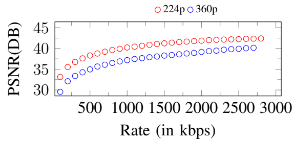
Figure 211. Curves of PSNR. Input: 360p, 2800Kbps
