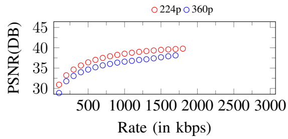
Figure 124. Curves of PSNR. Input: 360p, 1800Kbps
