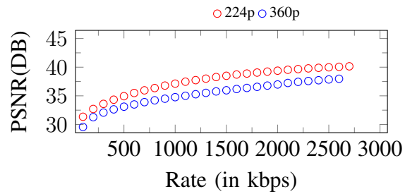
Figure 56. Curves of PSNR. Input: 360p, 2700Kbps
