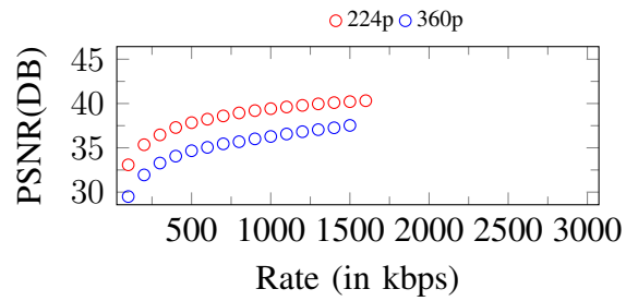
Figure 199. Curves of PSNR. Input: 360p, 1600Kbps
