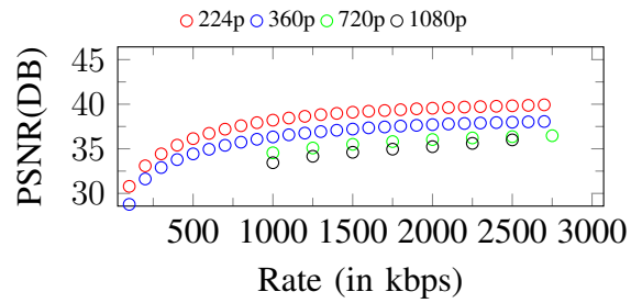
Figure 153. Curves of PSNR. Input: 1080p, 2750Kbps
