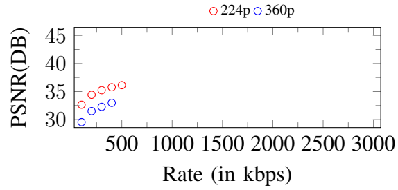
Figure 188. Curves of PSNR. Input: 360p, 500Kbps
