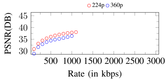
Figure 117. Curves of PSNR. Input: 360p, 1100Kbps
