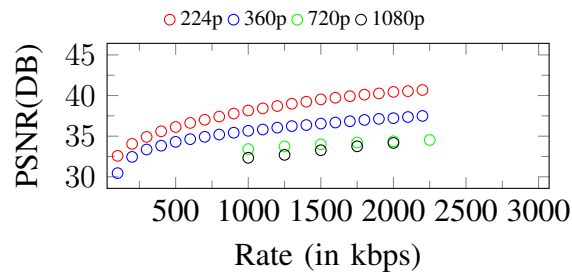
Figure 305. Curves of PSNR. Input: 1080p, 2250Kbps
