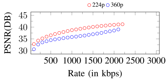
Figure 282. Curves of PSNR. Input: 360p, 2200Kbps
