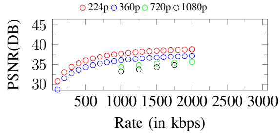
Figure 150. Curves of PSNR. Input: 1080p, 2000Kbps
