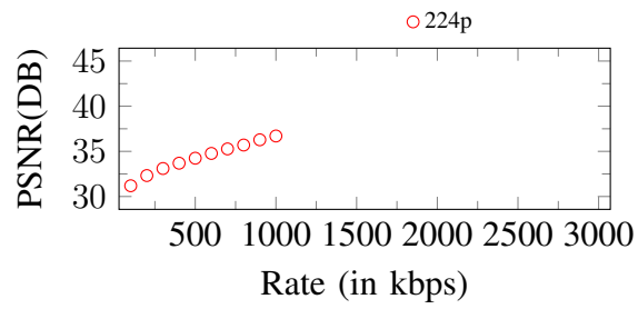
Figure 10. Curves of PSNR. Input: 224p, 1100Kbps
