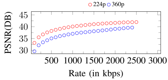
Figure 208. Curves of PSNR. Input: 360p, 2500Kbps
