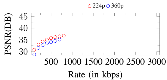
Figure 114. Curves of PSNR. Input: 360p, 800Kbps
