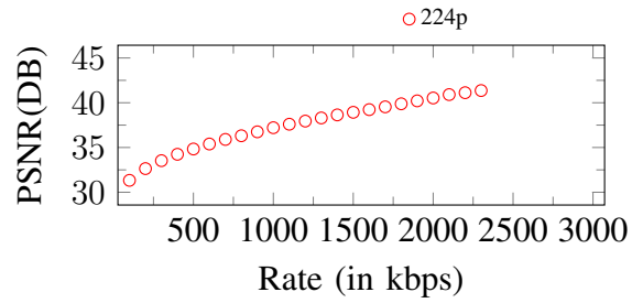
Figure 23. Curves of PSNR. Input: 224p, 2400Kbps
