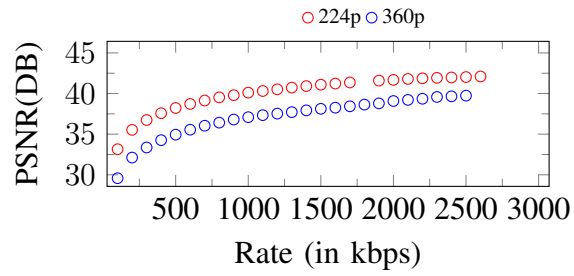
Figure 209. Curves of PSNR. Input: 360p, 2600Kbps
