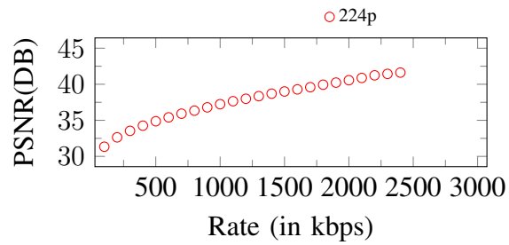
Figure 24. Curves of PSNR. Input: 224p, 2500Kbps
