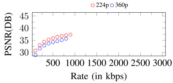
Figure 115. Curves of PSNR. Input: 360p, 900Kbps
