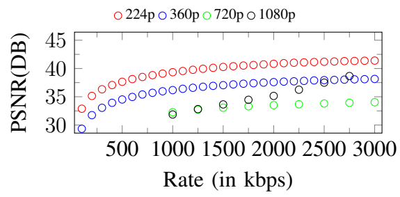
Figure 231. Curves of PSNR. Input: 1080p, 3000Kbps
