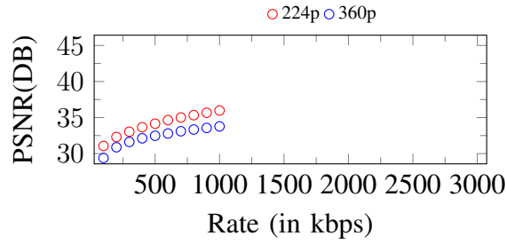
Figure 60. Curves of PSNR. Input: 720p, 1000Kbps
