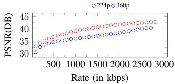
Figure 288. Curves of PSNR. Input: 360p, 2800Kbps
