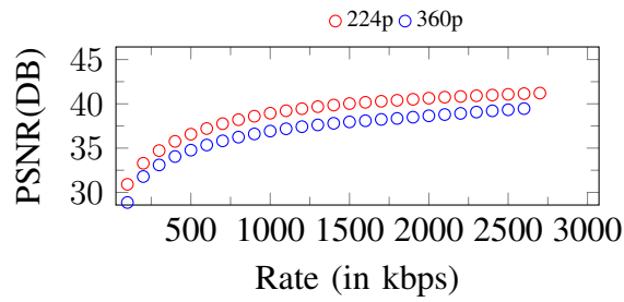
Figure 133. Curves of PSNR. Input: 360p, 2700Kbps
