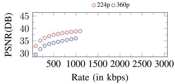
Figure 194. Curves of PSNR. Input: 360p, 1100Kbps
