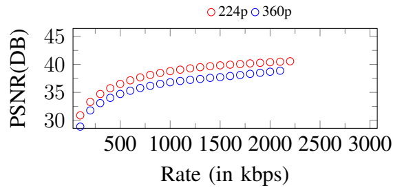
Figure 128. Curves of PSNR. Input: 360p, 2200Kbps
