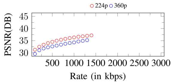
Figure 43. Curves of PSNR. Input: 360p, 1400Kbps
