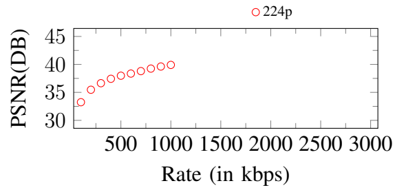
Figure 164. Curves of PSNR. Input: 224p, 1100Kbps
