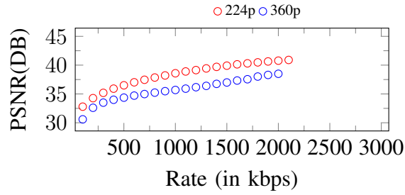
Figure 281. Curves of PSNR. Input: 360p, 2100Kbps
