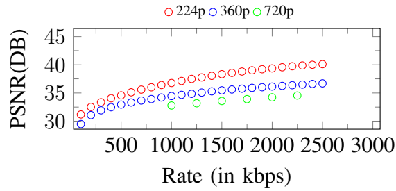
Figure 66. Curves of PSNR. Input: 720p, 2500Kbps
