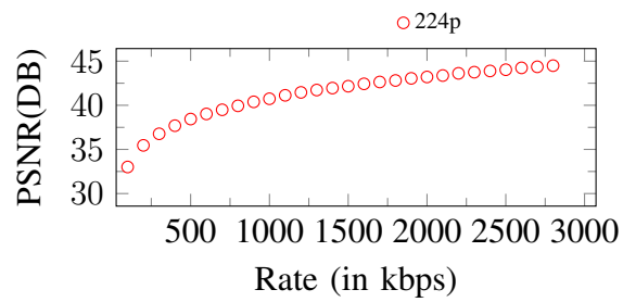
Figure 182. Curves of PSNR. Input: 224p, 2900Kbps
