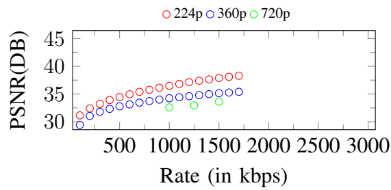
Figure 63. Curves of PSNR. Input: 720p, 1750Kbps
