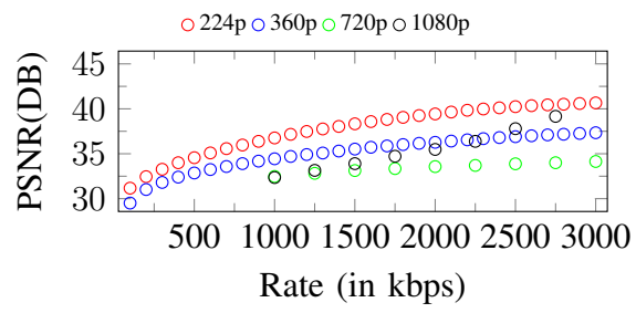
Figure 77. Curves of PSNR. Input: 1080p, 3000Kbps
