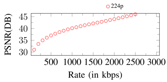
Figure 106. Curves of PSNR. Input: 224p, 3000Kbps
