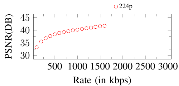
Figure 170. Curves of PSNR. Input: 224p, 1700Kbps
