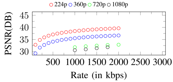
Figure 227. Curves of PSNR. Input: 1080p, 2000Kbps
