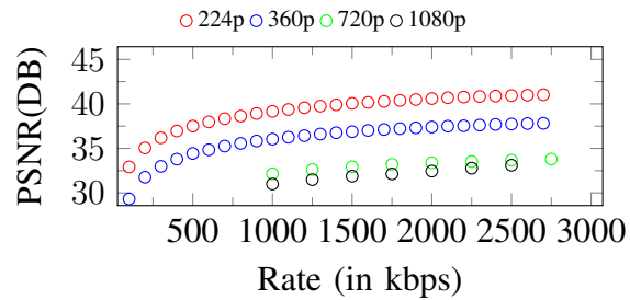
Figure 230. Curves of PSNR. Input: 1080p, 2750Kbps
