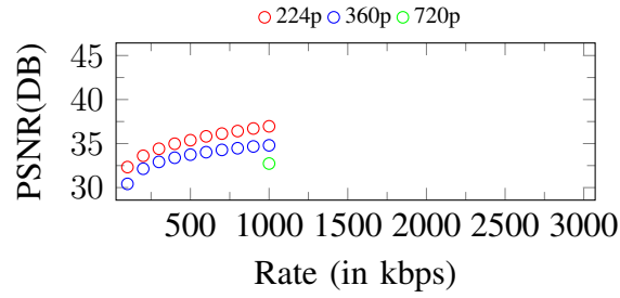
Figure 300. Curves of PSNR. Input: 1080p, 1000Kbps
