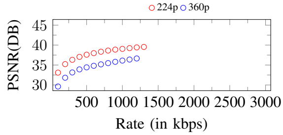
Figure 196. Curves of PSNR. Input: 360p, 1300Kbps
