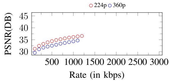
Figure 41. Curves of PSNR. Input: 360p, 1200Kbps
