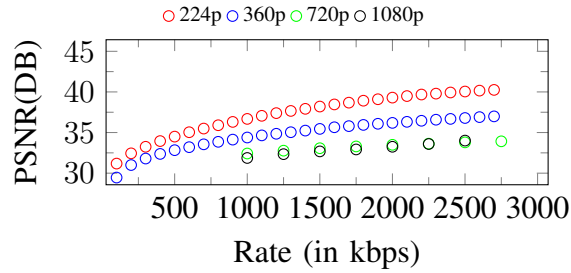
Figure 76. Curves of PSNR. Input: 1080p, 2750Kbps
