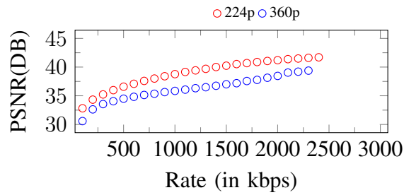
Figure 284. Curves of PSNR. Input: 360p, 2400Kbps
