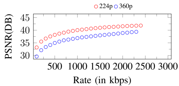
Figure 207. Curves of PSNR. Input: 360p, 2400Kbps
