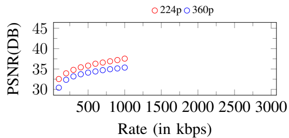
Figure 291. Curves of PSNR. Input: 720p, 1000Kbps
