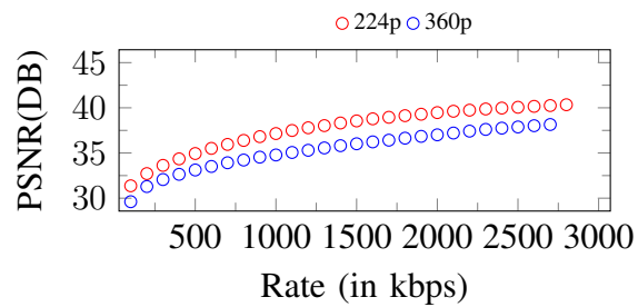
Figure 57. Curves of PSNR. Input: 360p, 2800Kbps
