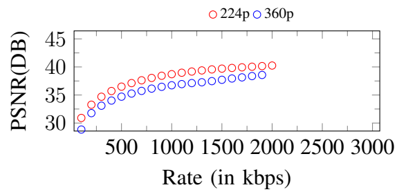
Figure 126. Curves of PSNR. Input: 360p, 2000Kbps
