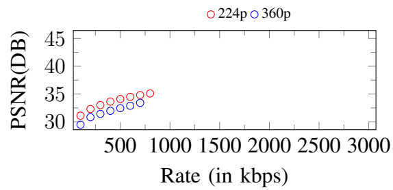
Figure 37. Curves of PSNR. Input: 360p, 800Kbps
