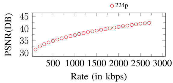
Figure 27. Curves of PSNR. Input: 224p, 2800Kbps
