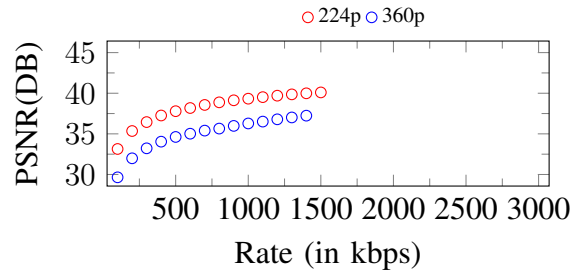
Figure 198. Curves of PSNR. Input: 360p, 1500Kbps
