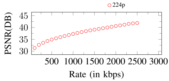
Figure 25. Curves of PSNR. Input: 224p, 2600Kbps
