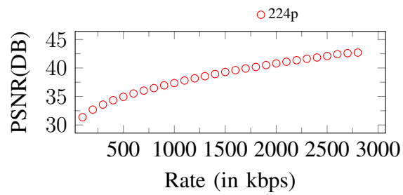
Figure 28. Curves of PSNR. Input: 224p, 2900Kbps
