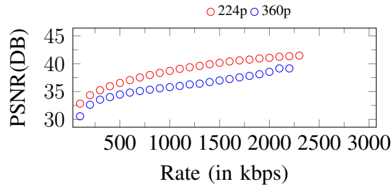
Figure 283. Curves of PSNR. Input: 360p, 2300Kbps
