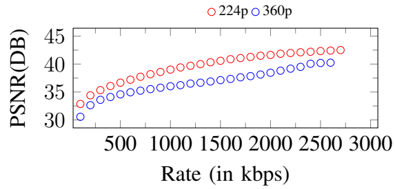
Figure 287. Curves of PSNR. Input: 360p, 2700Kbps
