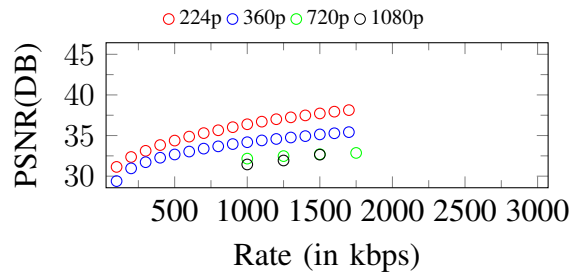
Figure 72. Curves of PSNR. Input: 1080p, 1750Kbps
