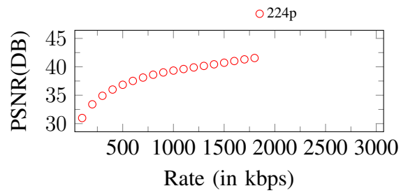
Figure 95. Curves of PSNR. Input: 224p, 1900Kbps
