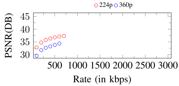
Figure 190. Curves of PSNR. Input: 360p, 700Kbps
