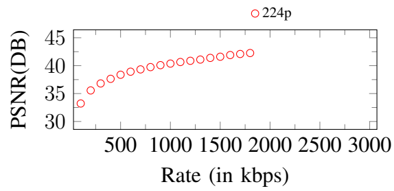
Figure 172. Curves of PSNR. Input: 224p, 1900Kbps
