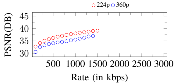
Figure 275. Curves of PSNR. Input: 360p, 1500Kbps
