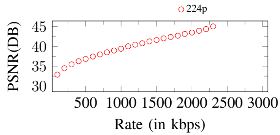
Figure 254. Curves of PSNR. Input: 224p, 2400Kbps
