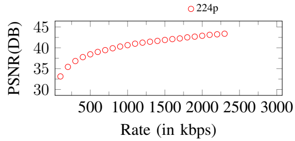
Figure 177. Curves of PSNR. Input: 224p, 2400Kbps
