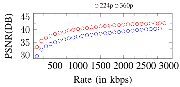
Figure 212. Curves of PSNR. Input: 360p, 2900Kbps
