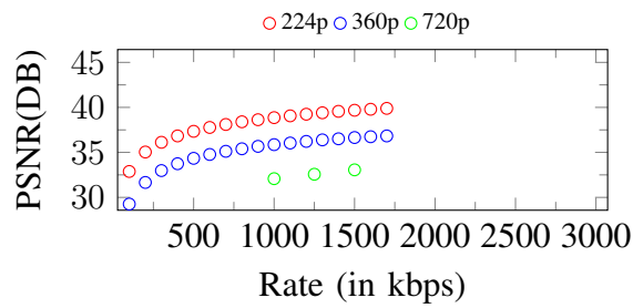
Figure 217. Curves of PSNR. Input: 720p, 1750Kbps
