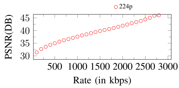
Figure 29. Curves of PSNR. Input: 224p, 3000Kbps
