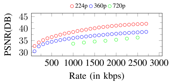
Figure 298. Curves of PSNR. Input: 720p, 2750Kbps
