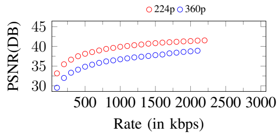
Figure 205. Curves of PSNR. Input: 360p, 2200Kbps
