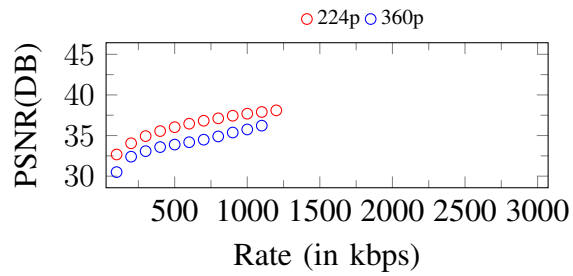
Figure 272. Curves of PSNR. Input: 360p, 1200Kbps
