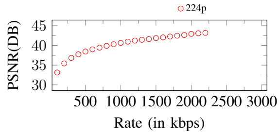
Figure 176. Curves of PSNR. Input: 224p, 2300Kbps
