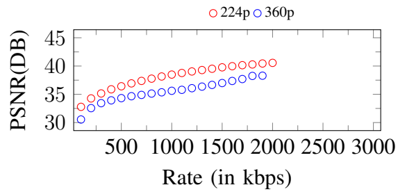
Figure 280. Curves of PSNR. Input: 360p, 2000Kbps
