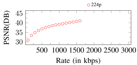
Figure 93. Curves of PSNR. Input: 224p, 1700Kbps
