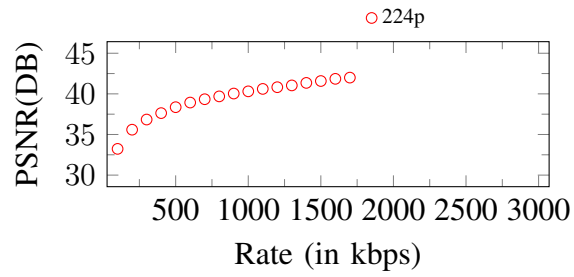
Figure 171. Curves of PSNR. Input: 224p, 1800Kbps
