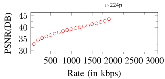
Figure 250. Curves of PSNR. Input: 224p, 2000Kbps
