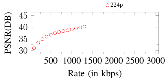
Figure 90. Curves of PSNR. Input: 224p, 1400Kbps
