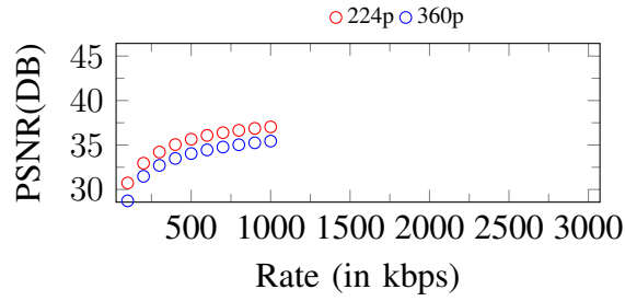
Figure 137. Curves of PSNR. Input: 720p, 1000Kbps
