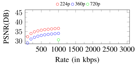
Figure 223. Curves of PSNR. Input: 1080p, 1000Kbps
