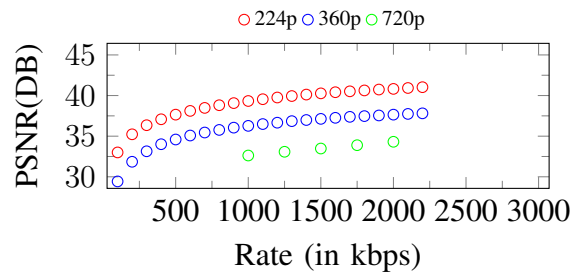
Figure 219. Curves of PSNR. Input: 720p, 2250Kbps
