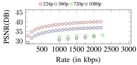
Figure 228. Curves of PSNR. Input: 1080p, 2250Kbps
