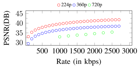
Figure 221. Curves of PSNR. Input: 720p, 2750Kbps
