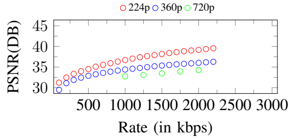
Figure 65. Curves of PSNR. Input: 720p, 2250Kbps
