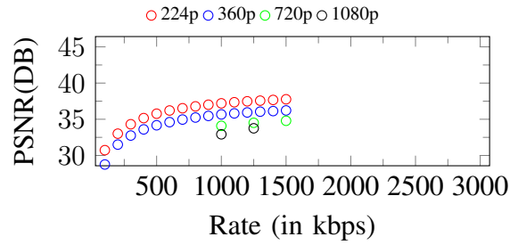
Figure 148. Curves of PSNR. Input: 1080p, 1500Kbps
