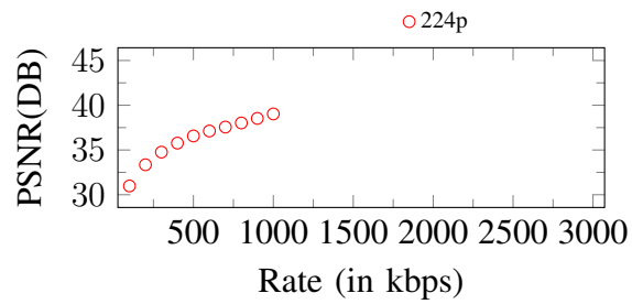
Figure 87. Curves of PSNR. Input: 224p, 1100Kbps
