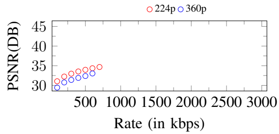
Figure 36. Curves of PSNR. Input: 360p, 700Kbps
