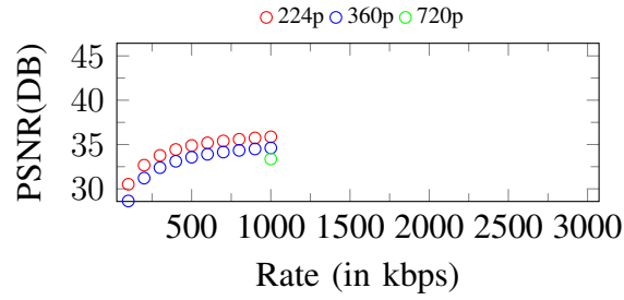
Figure 146. Curves of PSNR. Input: 1080p, 1000Kbps
