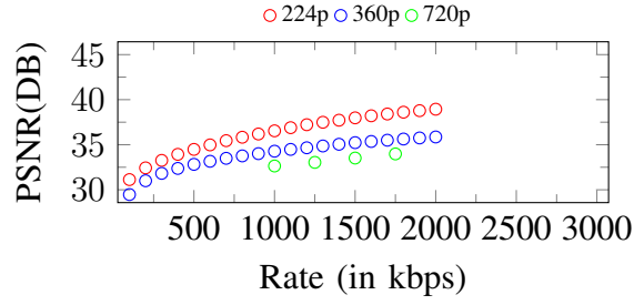
Figure 64. Curves of PSNR. Input: 720p, 2000Kbps
