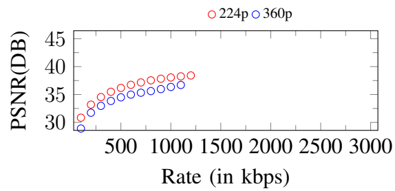
Figure 118. Curves of PSNR. Input: 360p, 1200Kbps
