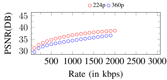
Figure 49. Curves of PSNR. Input: 360p, 2000Kbps
