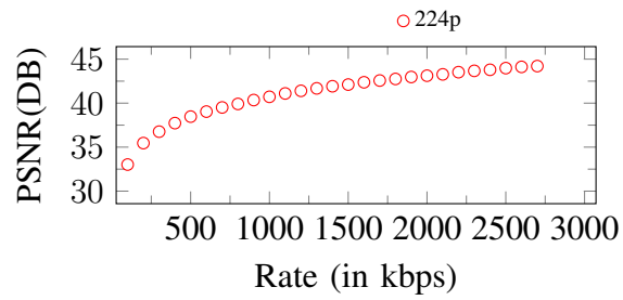
Figure 181. Curves of PSNR. Input: 224p, 2800Kbps
