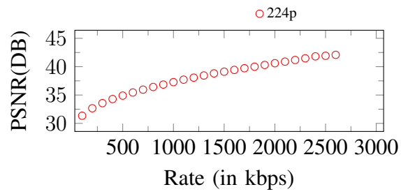
Figure 26. Curves of PSNR. Input: 224p, 2700Kbps
