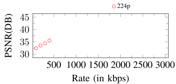
Figure 235. Curves of PSNR. Input: 224p, 500Kbps
