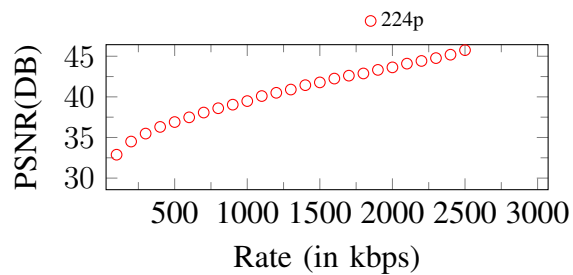
Figure 256. Curves of PSNR. Input: 224p, 2600Kbps
