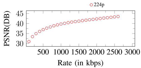
Figure 103. Curves of PSNR. Input: 224p, 2700Kbps
