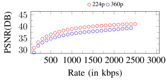
Figure 131. Curves of PSNR. Input: 360p, 2500Kbps
