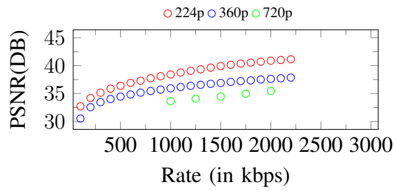
Figure 296. Curves of PSNR. Input: 720p, 2250Kbps
