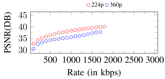
Figure 278. Curves of PSNR. Input: 360p, 1800Kbps
