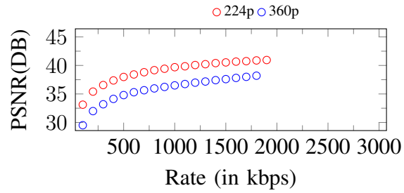
Figure 202. Curves of PSNR. Input: 360p, 1900Kbps
