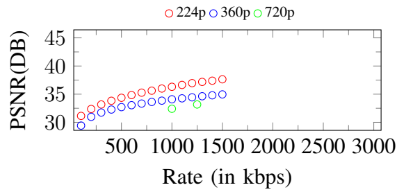
Figure 62. Curves of PSNR. Input: 720p, 1500Kbps
