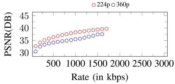
Figure 277. Curves of PSNR. Input: 360p, 1700Kbps
