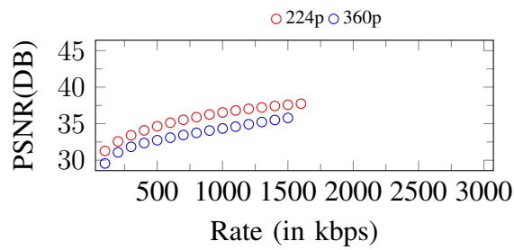
Figure 45. Curves of PSNR. Input: 360p, 1600Kbps
