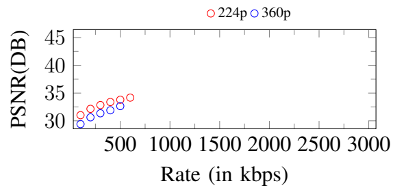
Figure 35. Curves of PSNR. Input: 360p, 600Kbps
