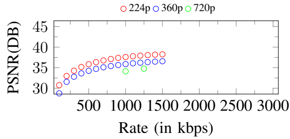
Figure 139. Curves of PSNR. Input: 720p, 1500Kbps
