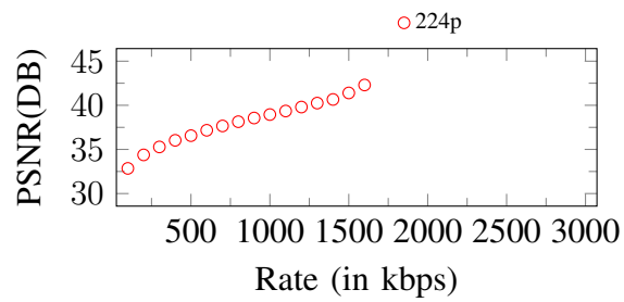
Figure 247. Curves of PSNR. Input: 224p, 1700Kbps
