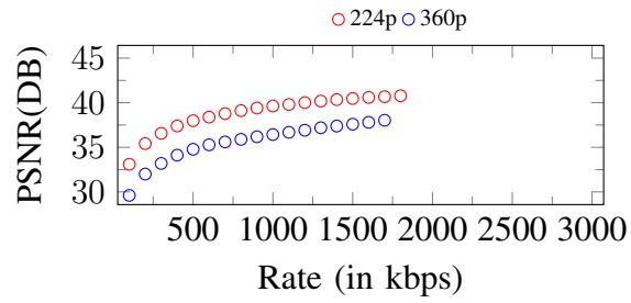
Figure 201. Curves of PSNR. Input: 360p, 1800Kbps
