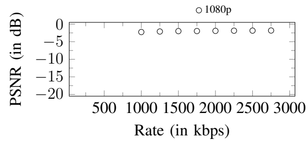
Figure 6. Up-scaling penalties curves. Original stream: 720p
