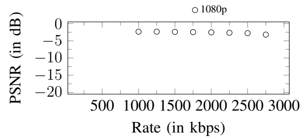
Figure 12. Up-scaling penalties curves. Original stream: 720p
