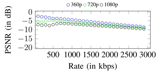
Figure 4. Up-scaling penalties curves. Original stream: 224p
