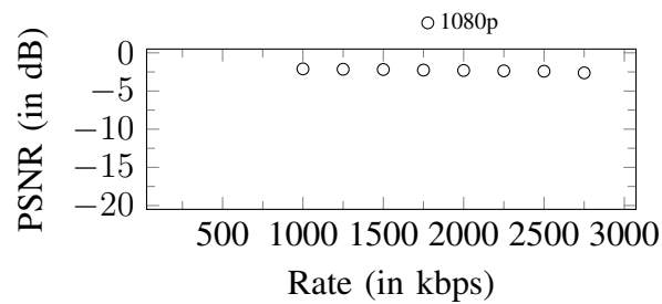
Figure 3. Up-scaling penalties curves. Original stream: 720p
