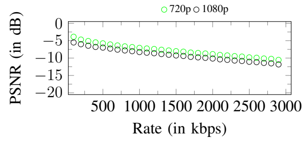
Figure 8. Up-scaling penalties curves. Original stream: 360p
