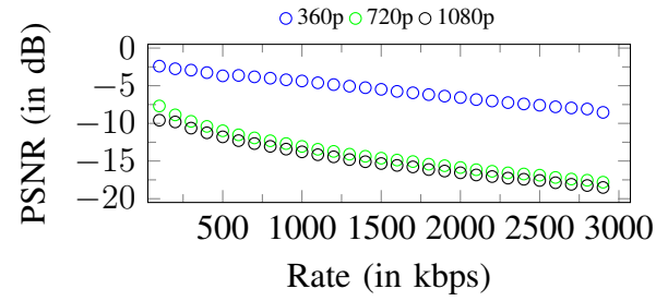
Figure 7. Up-scaling penalties curves. Original stream: 224p
