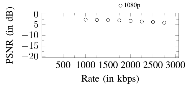
Figure 9. Up-scaling penalties curves. Original stream: 720p
