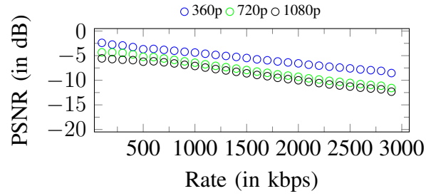
Figure 1. Up-scaling penalties curves. Original stream: 224p
