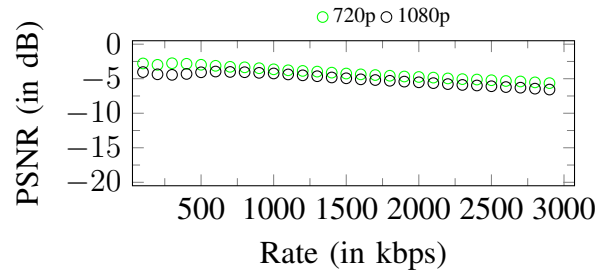
Figure 2. Up-scaling penalties curves. Original stream: 360p
