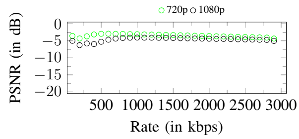
Figure 5. Up-scaling penalties curves. Original stream: 360p
