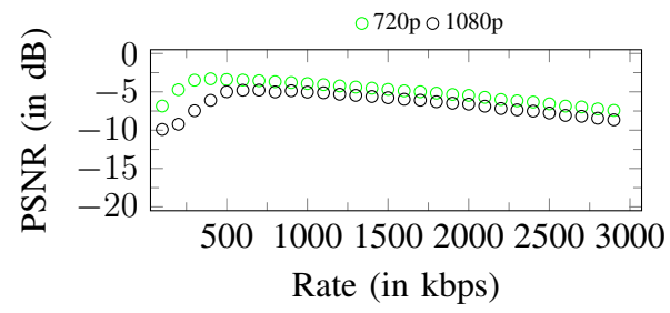
Figure 11. Up-scaling penalties curves. Original stream: 360p
