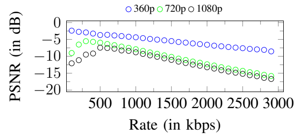
Figure 10. Up-scaling penalties curves. Original stream: 224p
